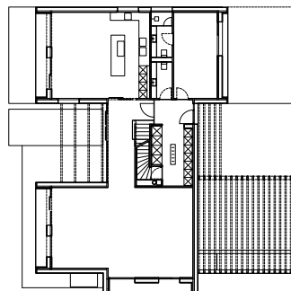
FIRST FLOOR 1:1000
